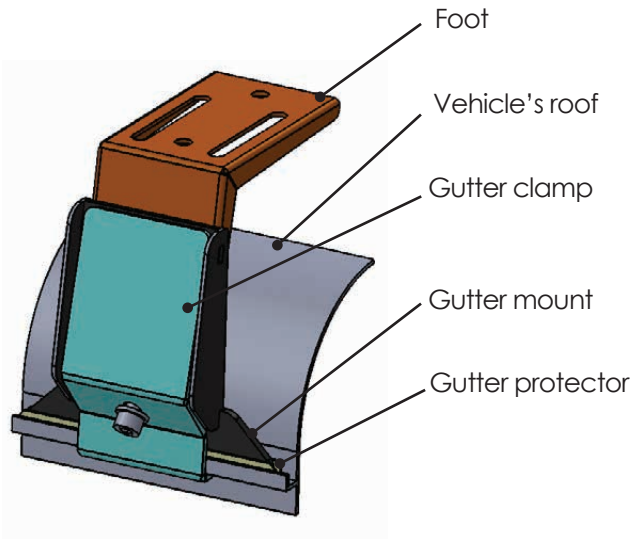
Typical Gutter Mount Layout
